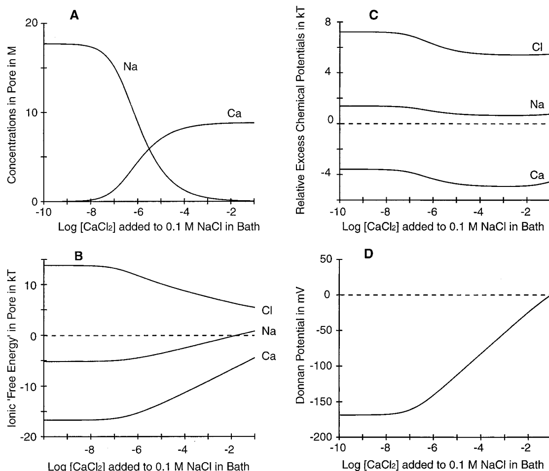
FIGURE 2 \text{Ca}^{2+} , \text{Na}^+ , and \text{Cl}^- selectivities in the hypothesized filter. In a simulated experiment, \text{CaCl}_2 is added to the 0.1 \text{ M NaCl} solution so the bath \text{Ca}^{2+} concentration is varied from 10^{-10} to 10^{-1} \text{ M} while \text{NaCl} remains at 10^{-1} \text{ M} . The selectivity filter is described using the standard pore of Fig. 1 A and the dielectric coefficient is assigned the value of 63.5. ( A ) Ionic concentrations in the selectivity filter. As bath \text{Ca}^{2+} is increased to micromolar concentrations, \text{Na}^+ is replaced by \text{Ca}^{2+} in the selectivity filter. The replacement is half complete at 1 \mu\text{M} bath \text{Ca}^{2+} (the dielectric coefficient was chosen to match this apparent dissociation constant). In this graph, the \text{Cl}^- curve is indistinguishable from the baseline. ( B ) Free energies of partitioning \Delta G_i for \text{Ca}^{2+} , \text{Na}^+ , and \text{Cl}^- vary as the ionic compositions in the bath (and hence the selectivity filter) are varied. \Delta G_i = \mu_i^{\text{ex}} - \mu_{0,i}^{\text{ex}} + z_i e_0 \Psi , where i identifies the type of ion and \Psi (note lower case) is the relative Donnan potential (filter/bath). ( C ) Differences of ionic excess chemical potentials (filter/bath) vary only weakly as \text{Ca}^{2+} replaces \text{Na}^+ in the selectivity filter. The offset between the (relative) excess chemical potential of \text{Ca}^{2+} and the (relative) excess chemical potential of \text{Na}^+ varies even less. ( D ) Donnan electric potential at the filter/bath junction varies strongly as \text{Ca}^{2+} replaces \text{Na}^+ in the selectivity filter. The variation in electrical potential has important effects on \text{Ca}^{2+}/\text{Na}^+ selectivity because the Donnan potential has differential effects on the electrical energy of divalent and monovalent ions. The free energy of \text{Ca}^{2+} partitioning ( panel B ) varies more strongly than that of \text{Na}^+ partitioning because the electrical energy of \text{Ca}^{2+} varies twice as much as the electrical energy of \text{Na}^+ .
